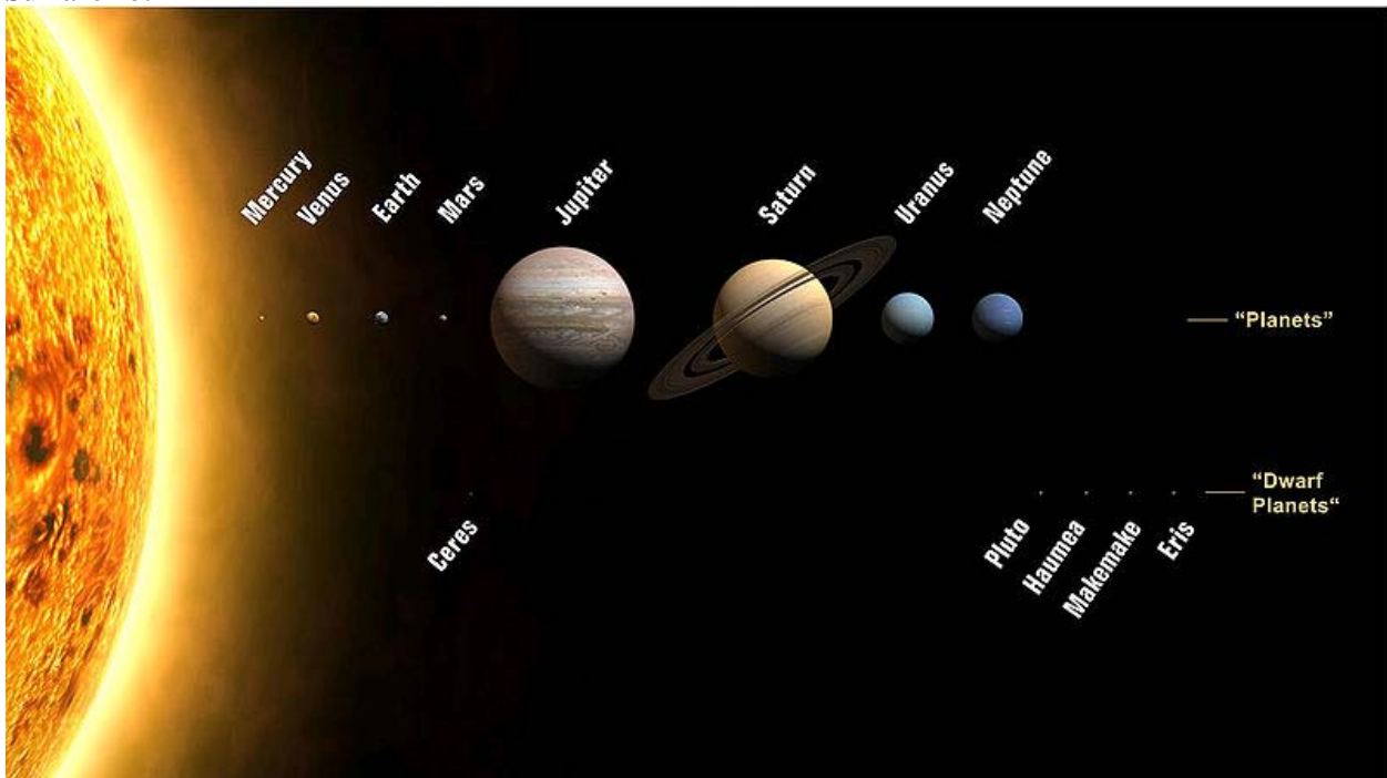
Figure 1 Planets and dwarf planets of the Solar System. Sizes are to scale, but relative distances from the Sun are not
